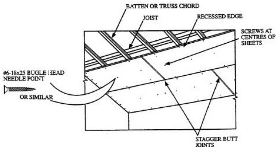
Ceiling Lining Fixing
