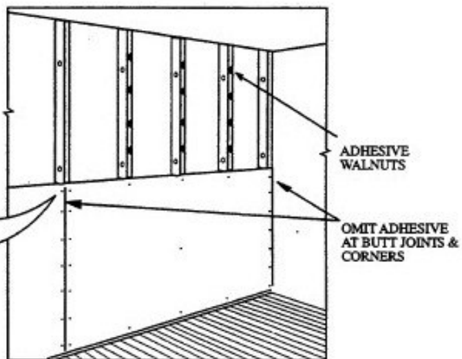
Wall Lining Fixing
